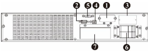
Diagramm 1: PowerWalker VFI 6000CRM LCD (L) Rückwand
