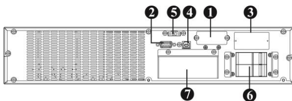
Diagram 1: Tylny panel PowerWalker VFI 6000CRM LCD (L)
