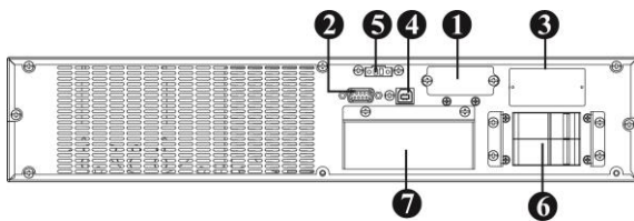
Diagram 1: PowerWalker VFI 6000CRM LCD (L) Rear Panel
