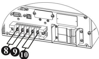
Diagram 2: Input/Output Terminal
