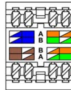
Two Row IDC Block Back View
