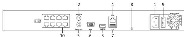
DS-608-8P
